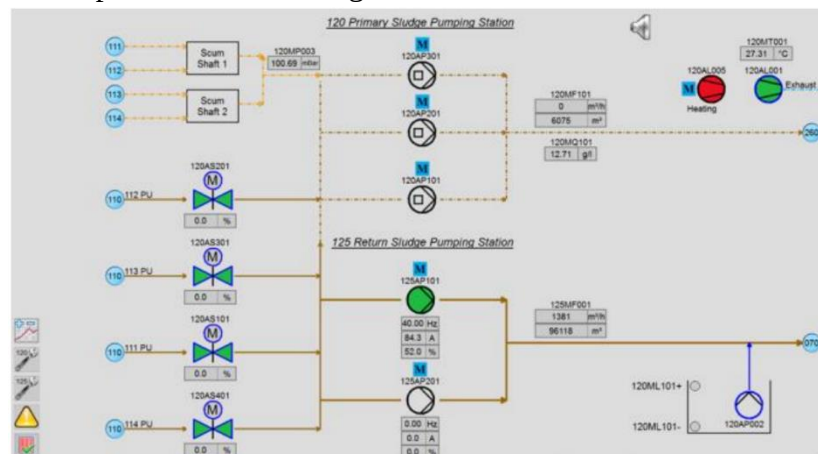
Fig. 6. Primary pumping stations of the wastewater treatment plant.
