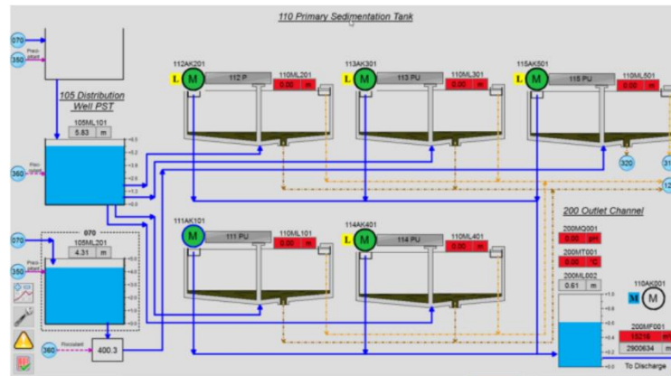
Fig. 5. Primary clarification of the wastewater treatment plant.
