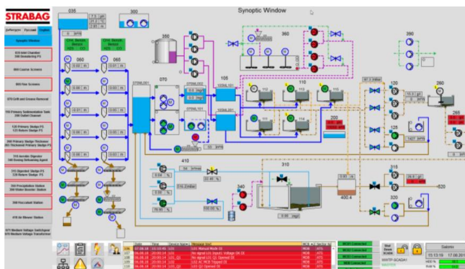
Fig. 7. Synoptic window of the wastewater treatment plant Gardabani.
