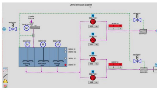
Fig. 4. Flocculant station of the wastewater treatment plant.
