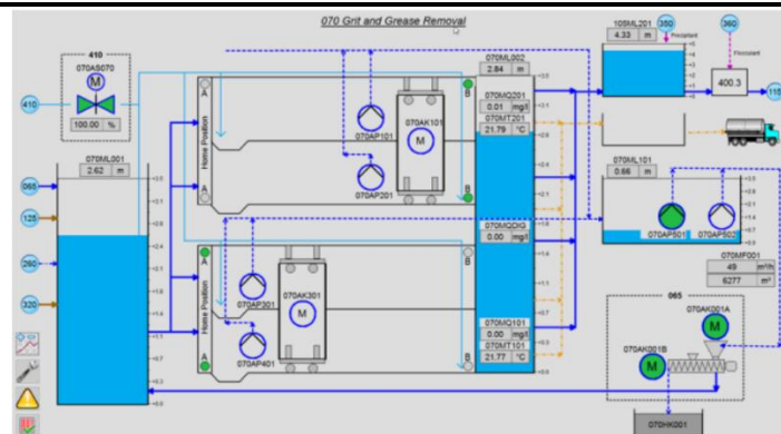
Fig. 3. Grit chambers of the wastewater treatment plant.
