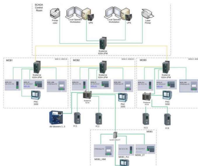
Fig. 8. General architecture for the SCADA SYSTEM GARDABANI.
