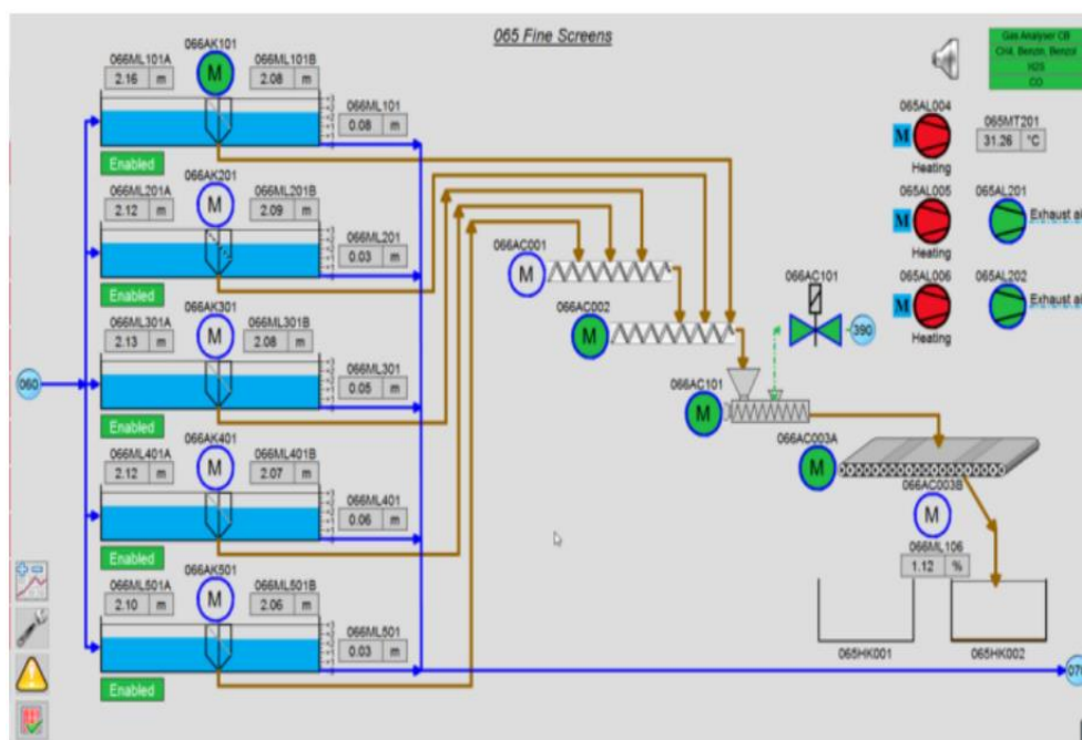
Fig. 2. Screens of the wastewater treatment plant.
