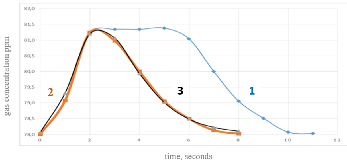
Fig.5. Diagram of changes in the amount of nitrogen gas in the drum.
