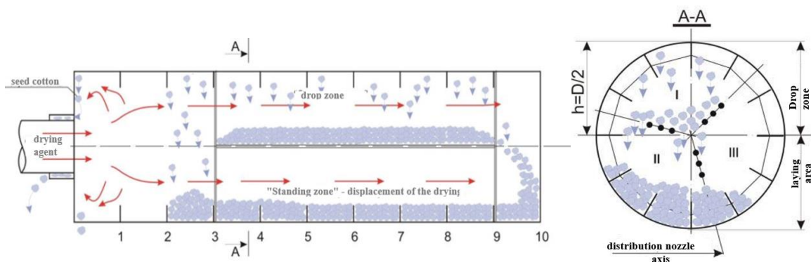
Fig.1. Distribution of raw cotton and drying agent along the length of the drum
